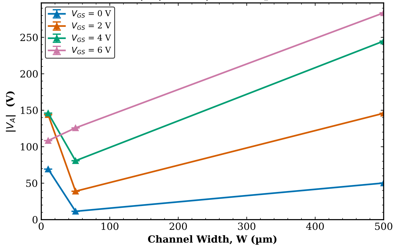
TFT1 Transistor 1 |V_A| vs W | L = 80\text{ }\mu\text{m}
